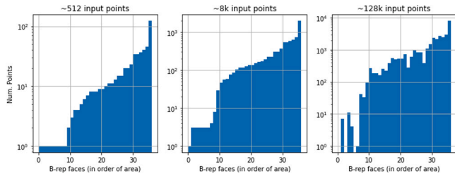
Fig. D.20. Histograms showing the number of points from each b-rep face which were used in at least one convolution, in a single MFCAD++ example. The maximum size of set \mathcal{N} has been set to 64. B-rep faces are sorted in order of surface areas. The input points were obtained with b-rep stratified sampling. Three input point cloud sizes are shown.
