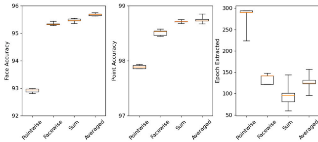
Fig. 5. Box plots showing multiple metrics on the MFCAD++ validation set achieved by different loss function configurations across five training runs. ‘Epoch extracted’ refers to the training epoch which achieved the maximum validation face accuracy during training — where model parameters were saved.
