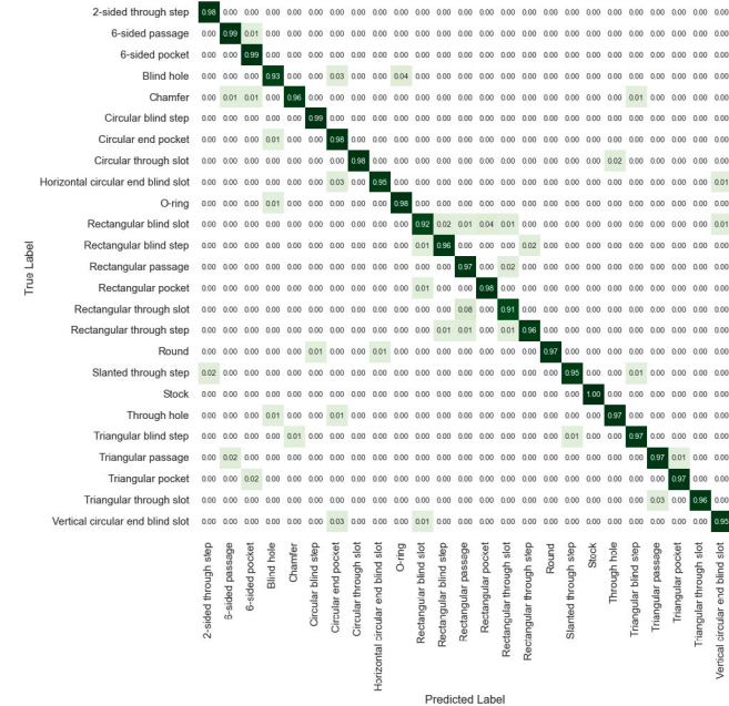
Fig. 9. Confusion matrix summarising the prediction accuracy of the final model configuration on the MFCAD++ dataset testing split.
