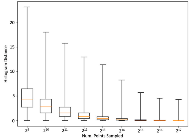
Fig. C.19. Box plots summarising the \chi^2 histogram distance of point distributions obtained by b-rep stratified sampling and simple random sampling, across the MFCAD++ validation set. For each point budget, each geometry is sampled once with each sampling method. The two point distributions obtained are then used to calculate a \chi^2 metric for each geometry. These values are then used to create the box plot for each point budget.
