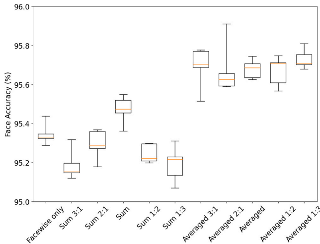
Fig. E.22. Box plot showing the different face labelling accuracies achieved by different total loss function configurations. The configuration with only pointwise loss has been omitted for clarity — it is significantly lower than the rest as shown in 5.
