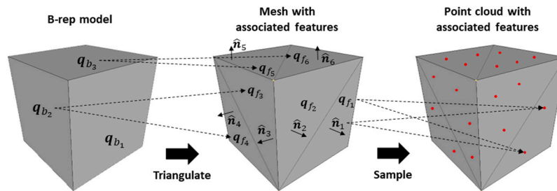
Fig. 3. Illustration of information flow from b-rep model to triangular mesh to point cloud. The chosen b-rep metadata, \mathbf{q}_b \in \mathbb{R}^D , is propagated to associated triangles. The inherited mesh triangle metadata, \mathbf{q}_f \in \mathbb{R}^D , is then also inherited by the sampled points; as well as the unit normal of the triangle, \hat{\mathbf{n}}_x .
