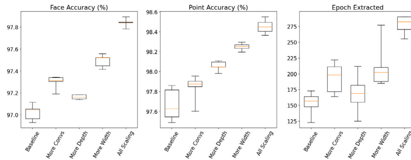
Fig. 8. Box plots showing multiple metrics on the MFCAD++ validation achieved by scaled configurations across five training runs.
