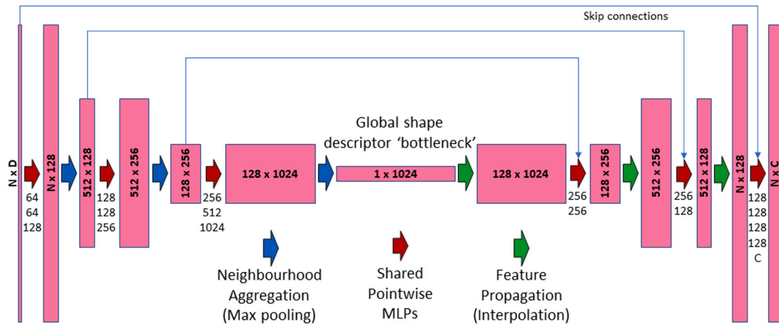
Fig. 2. Block diagram illustrating the baseline PointNet++ architecture. Arrangement and width of layers is shown. The bottleneck structure is also shown. N is the number of input points, D is the input feature dimension, and C is the number of classes.
