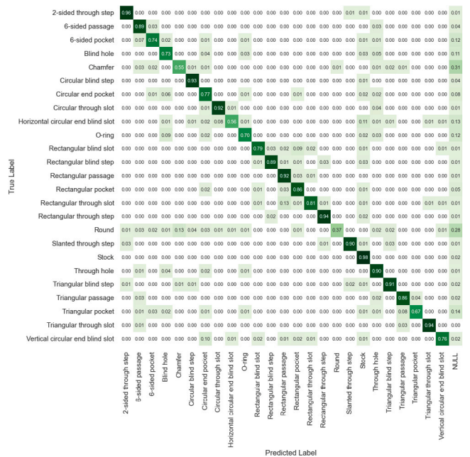
Fig. A.15. Confusion matrix for b-rep face predictions of a trained baseline model configuration.
