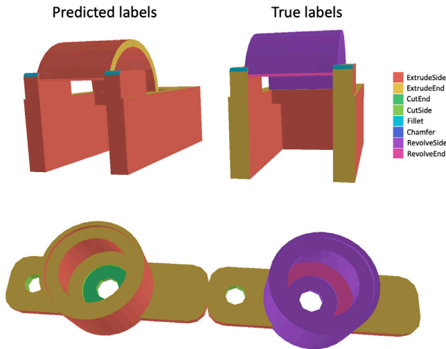
Fig. 13. Example of geometries where the model’s predictions are technically incorrect but are equally valid for creating the shape. (For interpretation of the references to colour in this figure legend, the reader is referred to the web version of this article.)
