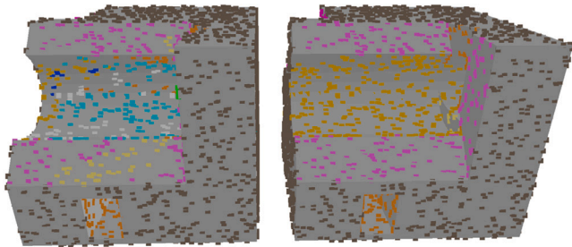
Fig. 6. Predicted point labels illustrated as colours, superimposed on the input CAD model. Both show the same set of points. The left points are coloured based on the direct predictions from the ‘pointwise’ branch. The right points are coloured based on predictions propagated from the ‘facewise’ branch. (For interpretation of the references to colour in this figure legend, the reader is referred to the web version of this article.)
