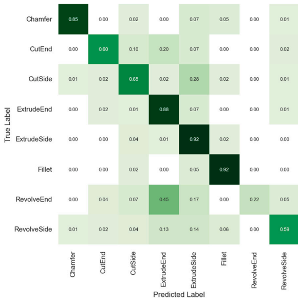
Fig. 12. Confusion matrix summarising the prediction accuracy of the final model configuration on the Fusion 360 Gallery segmentation dataset testing split.
