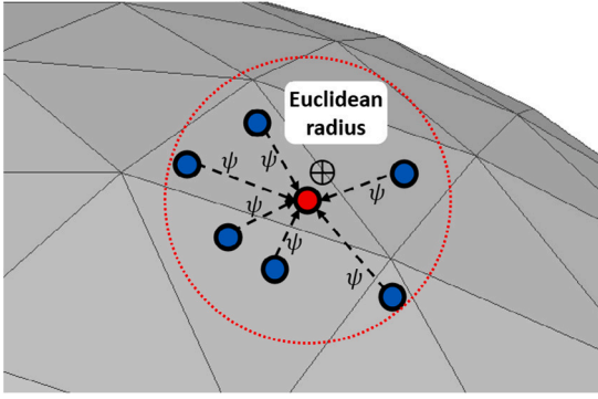
Fig. 1. Illustration of point convolution. Aggregating points within a Euclidean neighbourhood — an implicit local graph.
