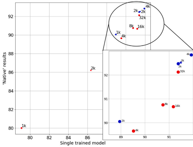
Fig. B.17. Evaluated b-rep face labelling accuracy of a single trained model with different sampling strategies against the accuracy of models trained and evaluated on the ‘native’ resolution. Data in red are simple random sampling and in blue are using b-rep stratified sampling. Solid circles use a maximum of 64 point neighbours during point convolution while starred data use 128. Data points are annotated with point cloud size. (For interpretation of the references to colour in this figure legend, the reader is referred to the web version of this article.)
