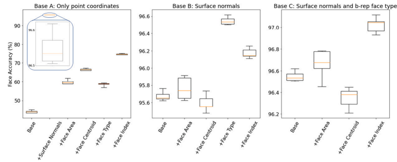
Fig. 7. Box plots showing the face labelling accuracy on the MFCAD++ validation set of different configurations. Each plot starts with a base configuration and adds input attributes separately.
