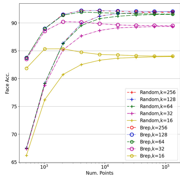
Fig. 4. Validation set performance of a single trained model when faced with different point sampling configurations. Simple random sampling and b-rep stratified sampling is shown across a range of point cloud sizes. Different maximum point neighbourhood sizes are also shown. (For interpretation of the references to colour in this figure legend, the reader is referred to the web version of this article.)
