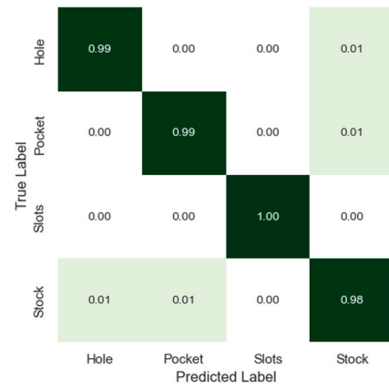
Fig. 10. Confusion matrix summarising the prediction accuracy of the final model configuration on the Zhang et al. machining features dataset testing split.
