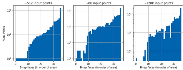
Fig. D.21. Histograms showing the number of points from each b-rep face which were used in at least one convolution, in a single MFCAD++ example. The maximum size of set \mathcal{N} has been set to 16. B-rep faces are sorted in order of surface areas. The input points were obtained with b-rep stratified sampling. Three input point cloud sizes are shown.
