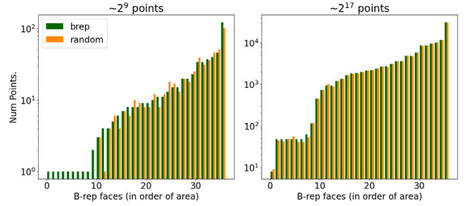
Fig. C.18. Histograms showing the number of points sampled from each b-rep face in a single MFCAD++ example. B-rep faces are sorted in order of surface areas. The distribution resulting in using b-rep stratified sampling and simple random sampling are shown side-by-side for comparison. Two input point cloud sizes are also shown for comparison. (For interpretation of the references to colour in this figure legend, the reader is referred to the web version of this article.)
